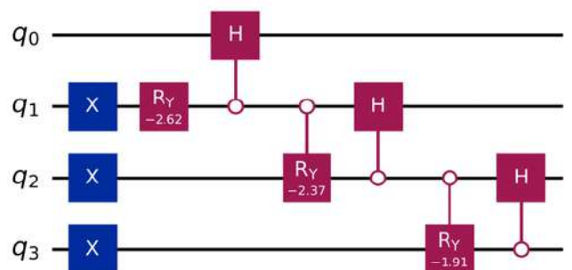
Figure 4: Quantum Circuits to Obtain the Uniform Superposition States (M=15)
