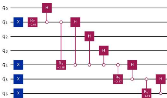
Figure 5: Quantum Circuits to Obtain the Uniform Superposition States (M=115)
